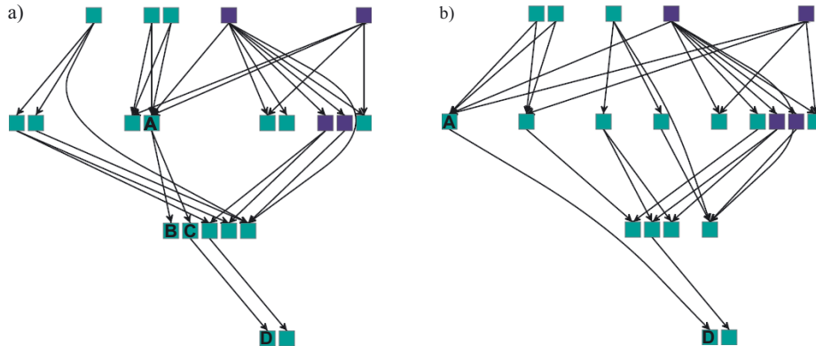
Fig. 2. Call graphs before and after a refactoring: The labeled nodes represent the following functions: A is DiffParser.getResult() , B is DiffParser.parseItCPP() , C is DiffParser.parseIt() and D is DiffType.getDiffNumber() . The colors of the nodes encode the package to which the method belongs.
